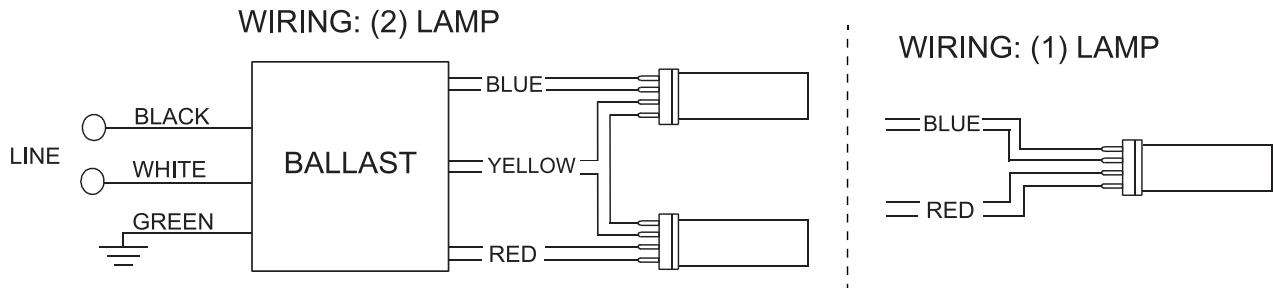
Figure 2 - Wiring Diagram
