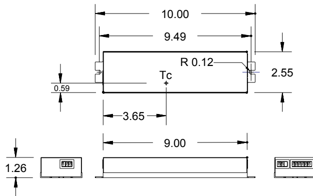
Figure 1 - Dimensional Data
