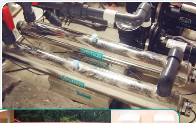
University Koi Pond and Fountain Water Treatment
