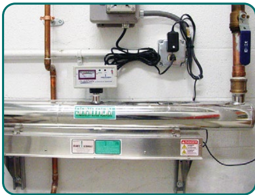
SANITRON® S50C on a Recirculation Water System
