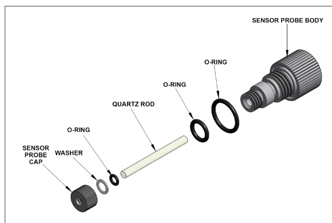
Figure 10 – Sensor Probe
