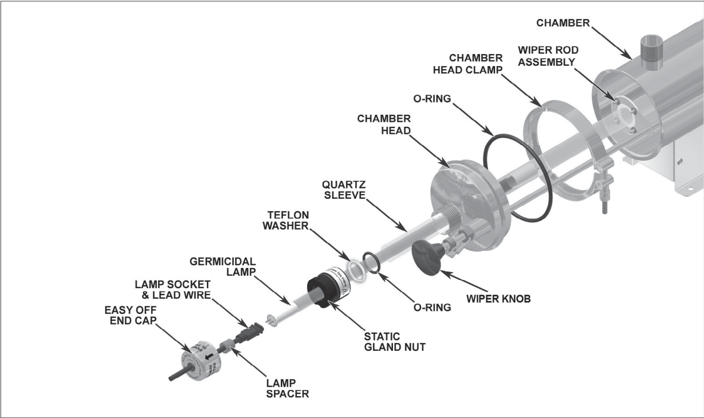
Figure 4 – Initial Installation of Quartz Sleeve
