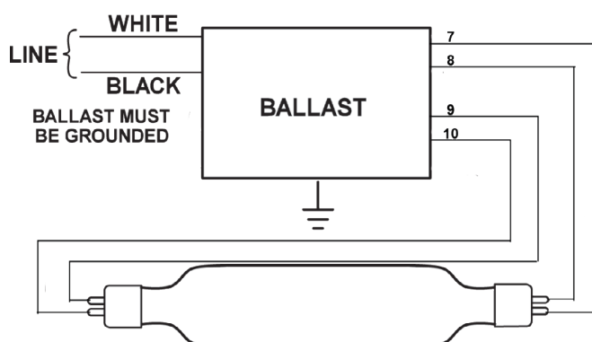
Wiring Diagram 1
