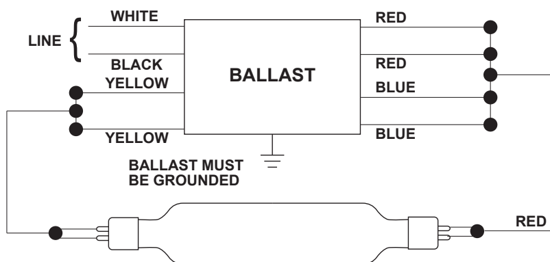
Wiring Diagram 1
